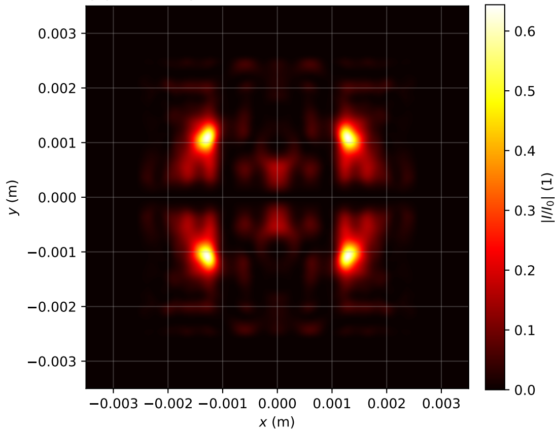
Intensity profile I(x, y, z = 3.901)/I_0 , P_{in}=8.0P_{cr} , artificial time
